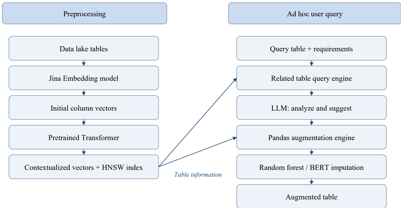
Figure 3-3. Backend software workflow.
