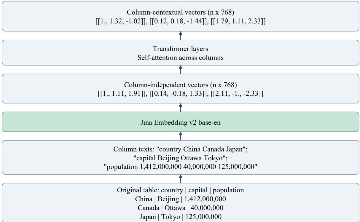
Figure 3-5. Model architecture.
