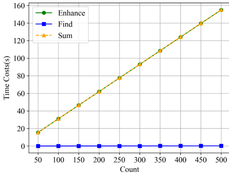
Figure 4-9. SDASDL processing-time curves for different numbers of tables.
