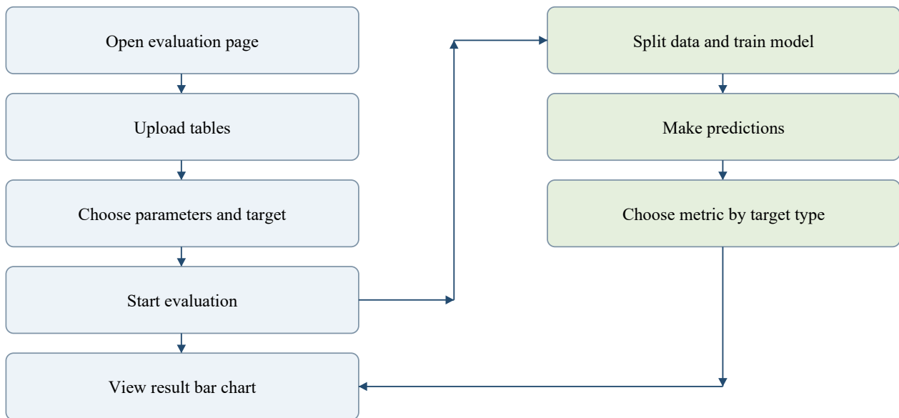
Figure 4-6. Downstream task evaluation workflow.
