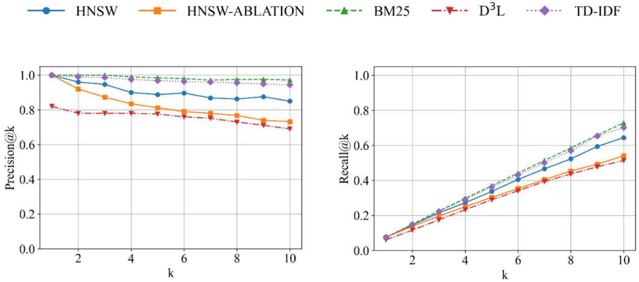
(a) P@k on Santos small. (b) R@k on Santos small.
