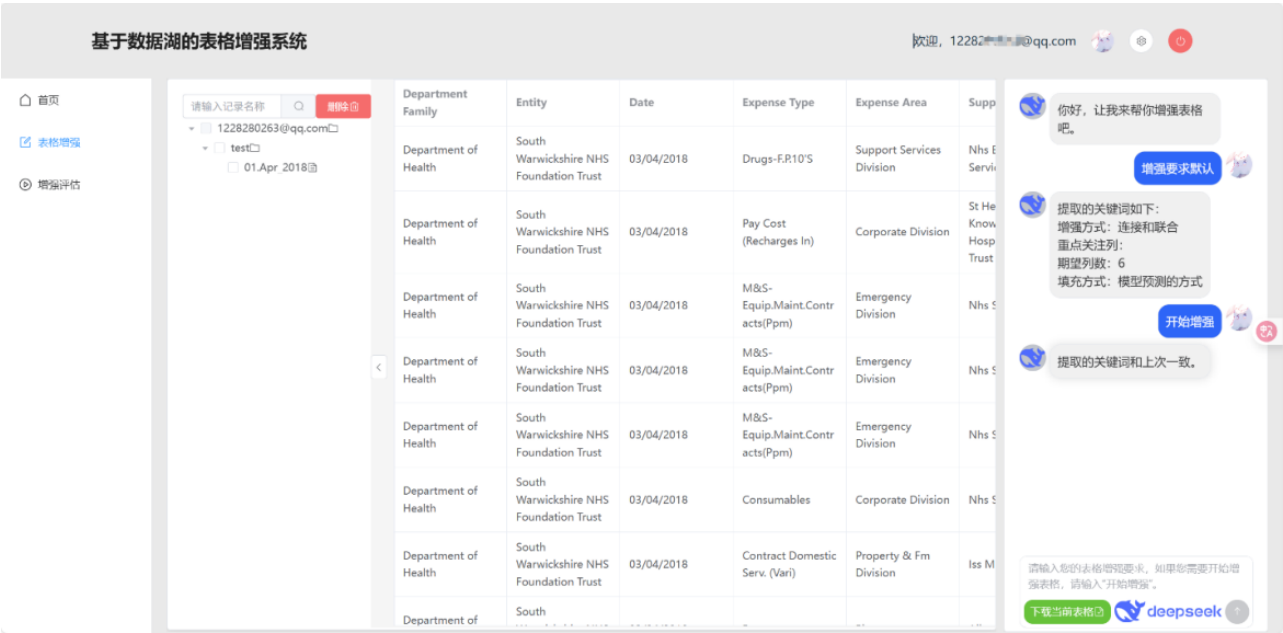
Figure 4-2. Table augmentation interface. Left: augmentation history. Center: query-table data. Right: conversation and augmentation requirements.
