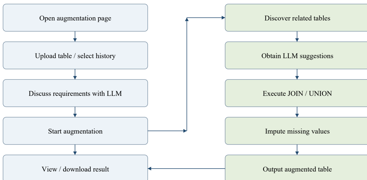
Figure 4-3. Table augmentation workflow.
