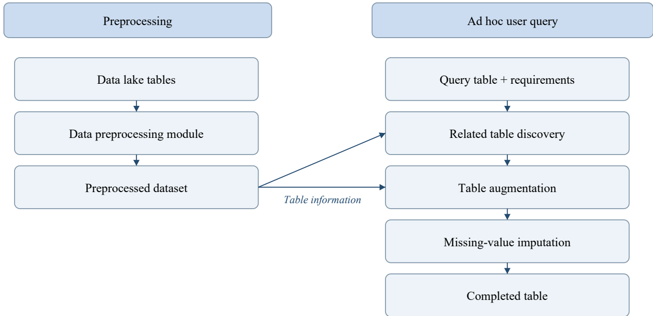
Figure 3-2. Backend system architecture.
