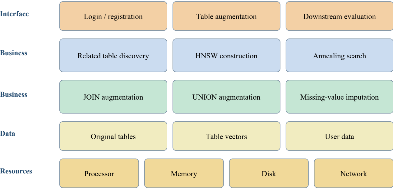
Figure 3-1. System architecture design.
