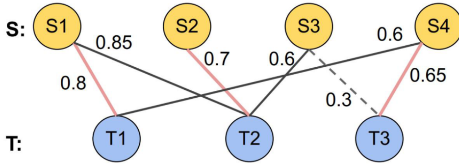
Figure 3-6. Example of table-similarity computation.
